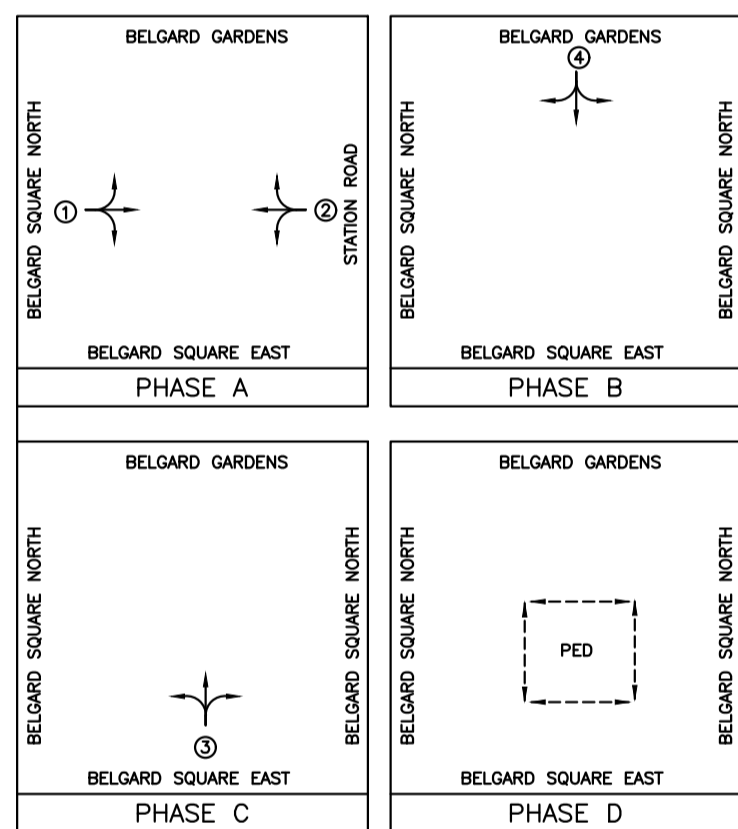
PROPOSED TRAFFIC SIGNALS STAGE DIAGRAM
